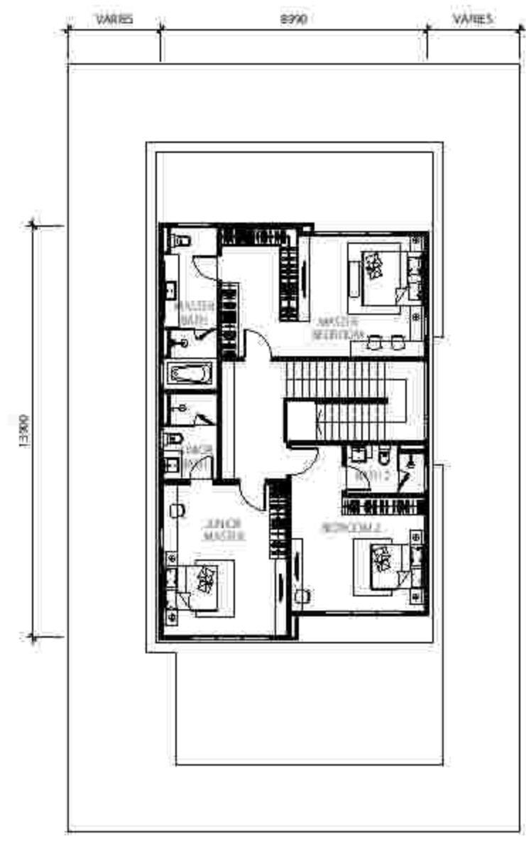
FIRST FLOOR
