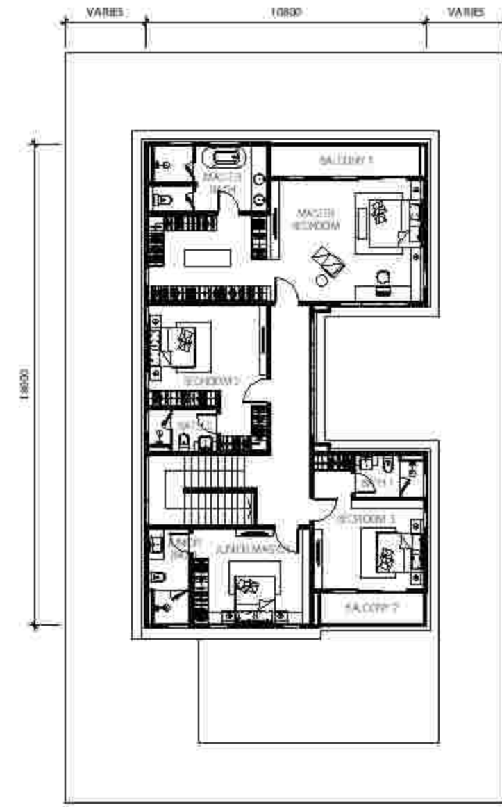
FIRST FLOOR
