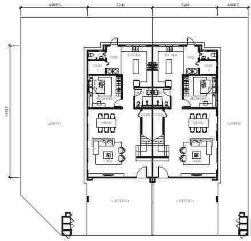
GROUND FLOOR | TYPE SD5D2a | TYPE SD5D1 Column | Intermediate
