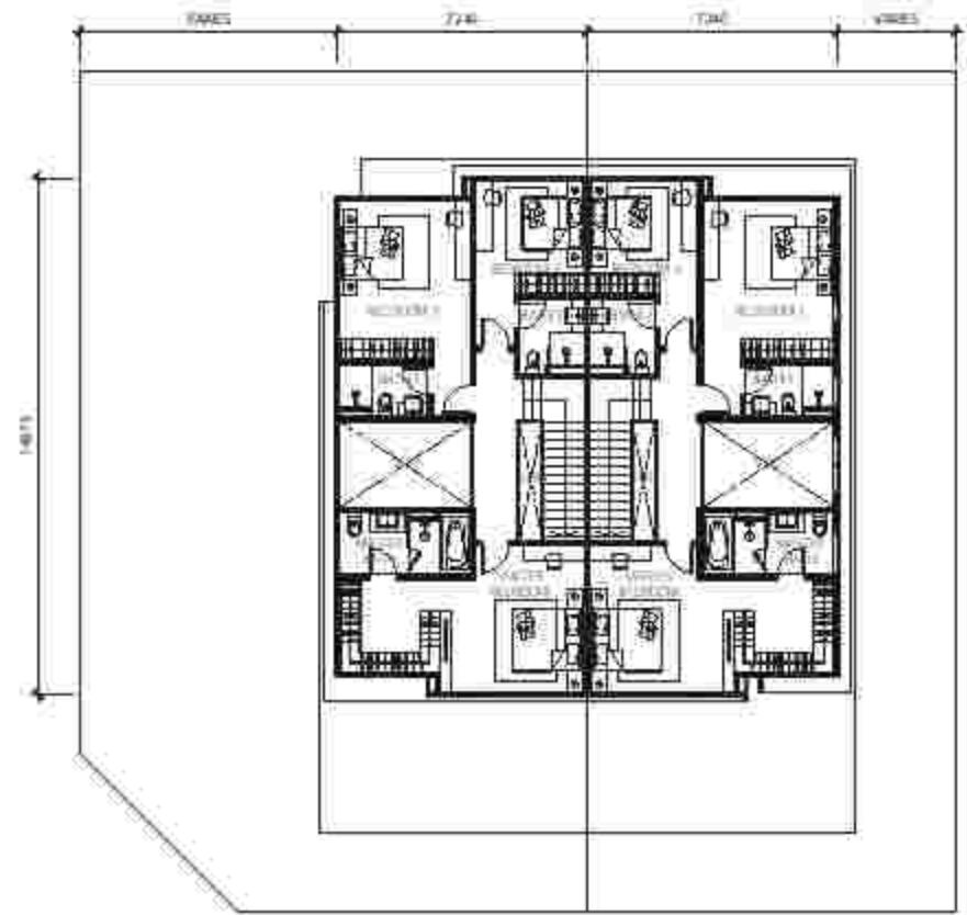
FIRST FLOOR | TYPE SD5C2a | TYPE SD5C1 Corridor | Intermediate
