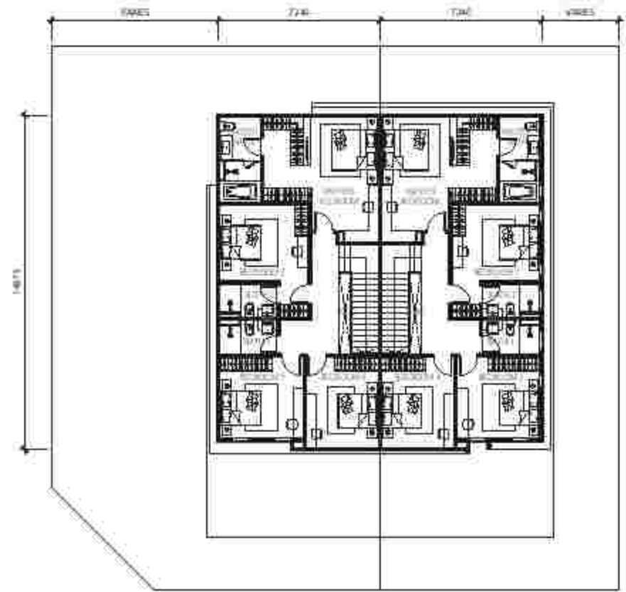
FIRST FLOOR | TYPE SD5D2a | TYPE SD5D1 Column | Intermediate
