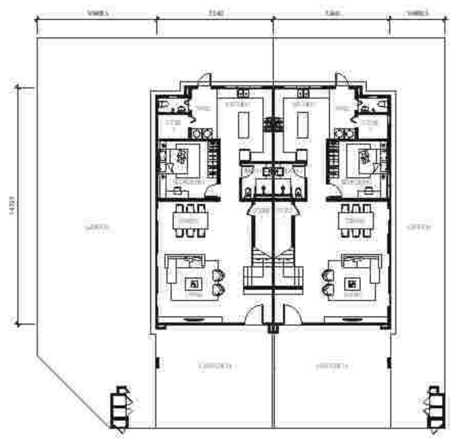
GROUND FLOOR | TYPE SD5C2a | TYPE SD5C1 Corridor | Intermediate
