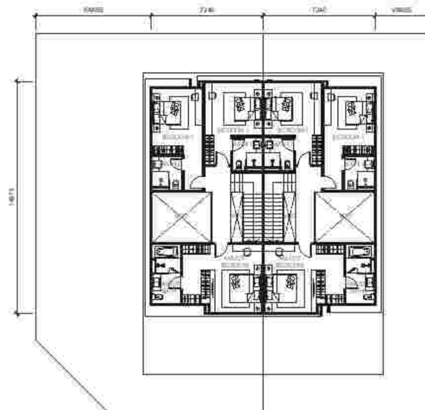
FIRST FLOOR | TYPE SD5A2a | TYPE SD5A1 Corridor | Intermediate
