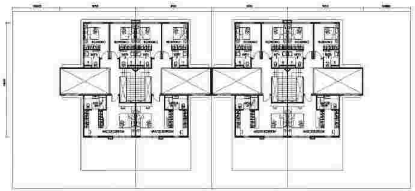
TYPE GH5D5a End
