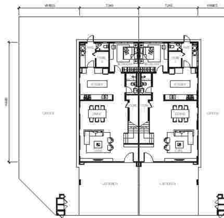
GROUND FLOOR | TYPE SD5A2a | TYPE SD5A1 Corridor | Intermediate
