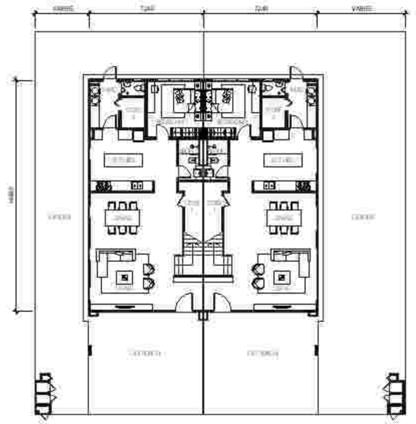
GROUND FLOOR | TYPE SD5B1a | TYPE SD5B3 Intermediate | End
